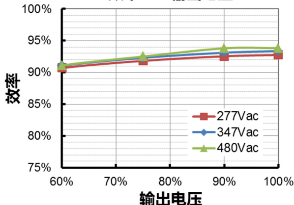
ESD-600S980DV( I_o=9800mA )
