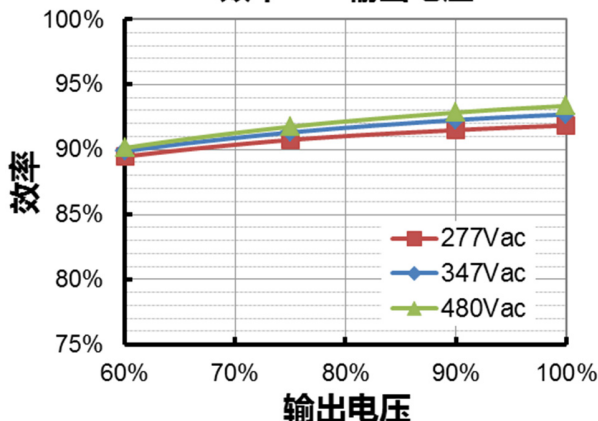
ESD-600S12ADV( I_o=12500mA )
