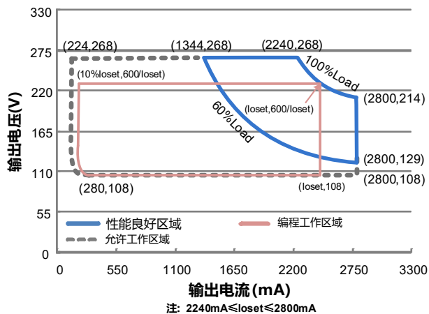
ESD-600S560DV
