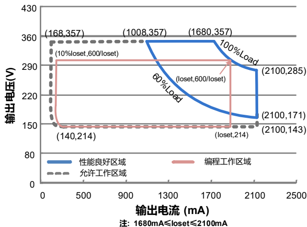
ESD-600S210DV
