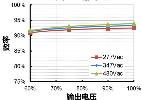
ESD-600S12ADV( I_o=10000mA )
