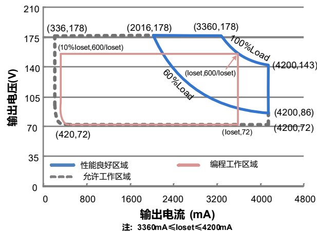
ESD-600S740DV
