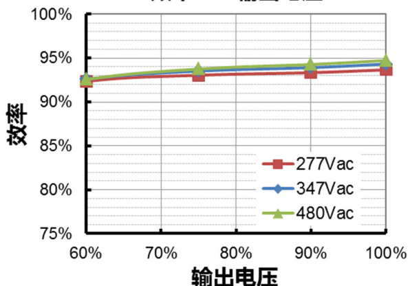
ESD-600S980DV( I_o=7840mA )
