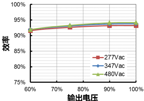
ESD-600S12ADV( I_o=10000mA )
