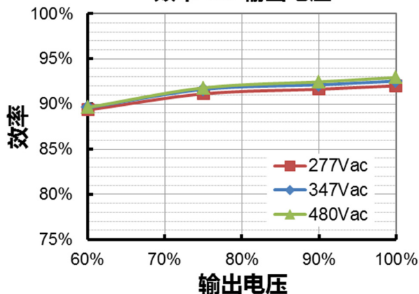
ESD-600S12ADV( I_o=12500mA )
