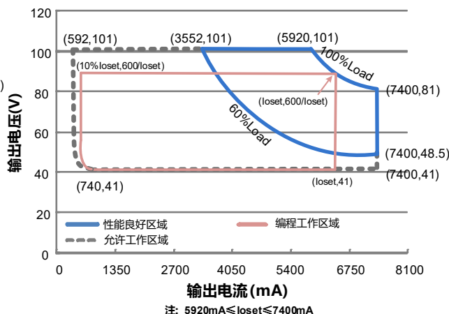
ESD-600S740DV
